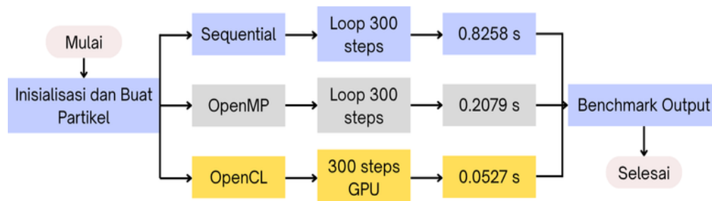
Gambar 1. Flowchart Sistem
